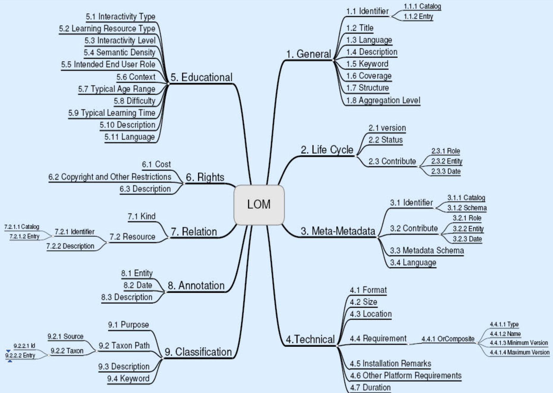
a schematic representation of the hierarchy of elements in the LOM data model
